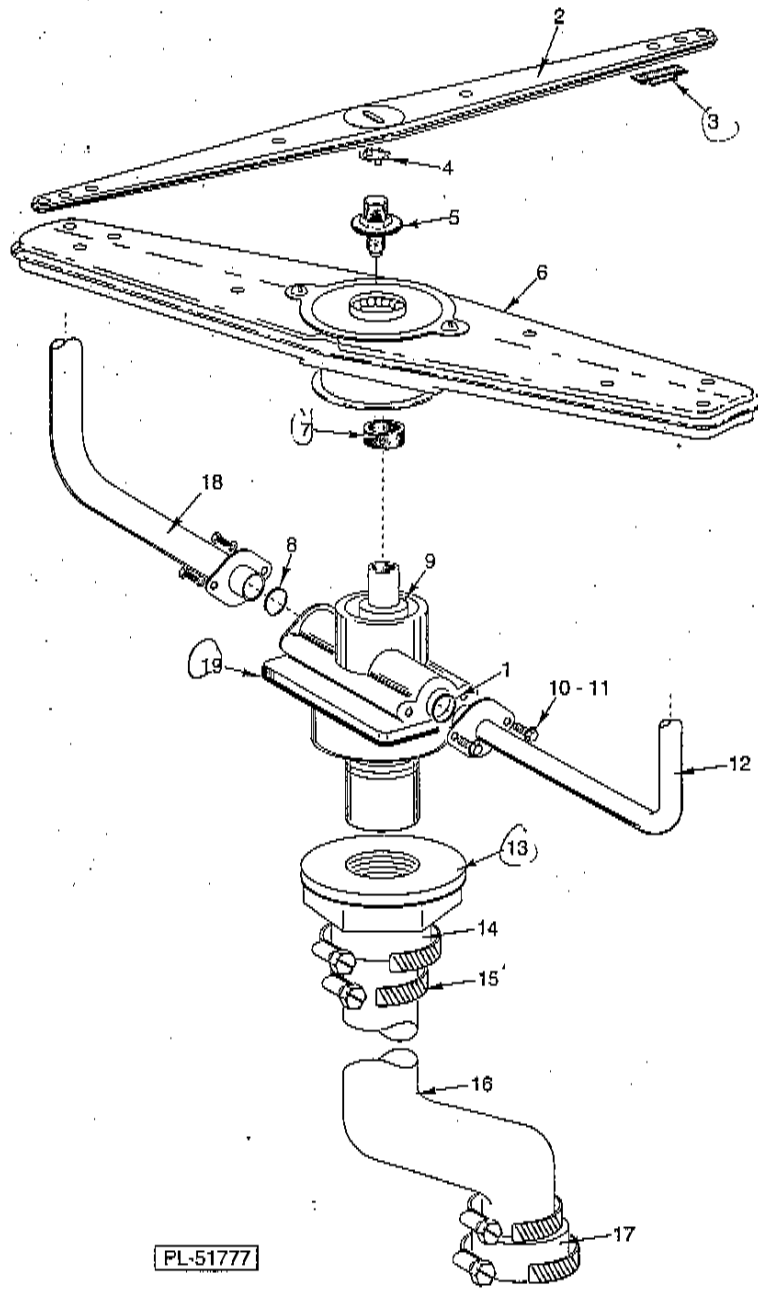
LOWER WASH & RINSE ARMS
