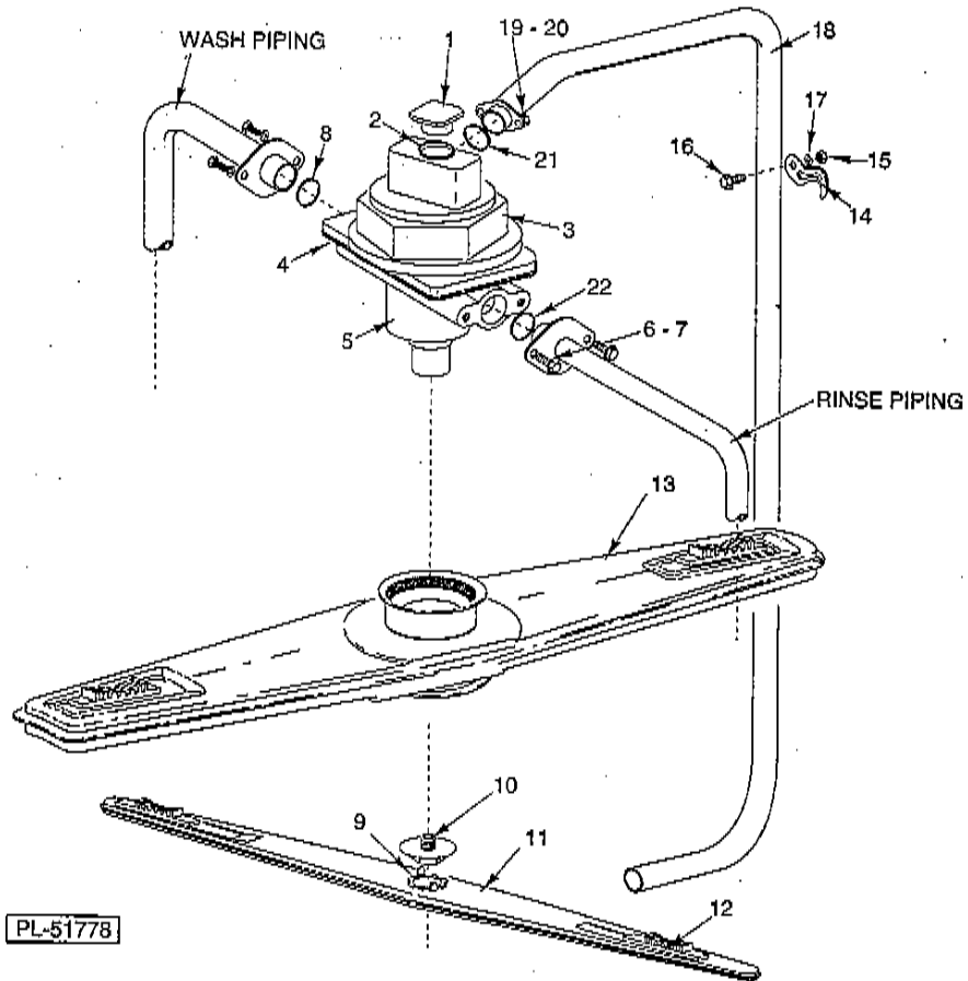
UPPER WASH & RINSE ARMS
