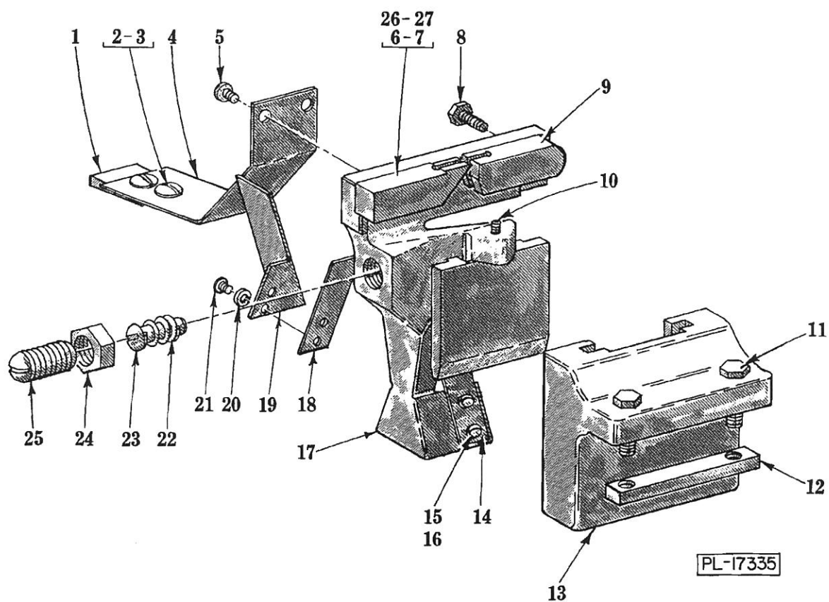
LOWER GUIDE AND WIPER UNIT
