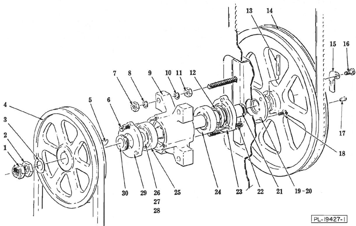
LOWER BEARING CARRIER UNIT
