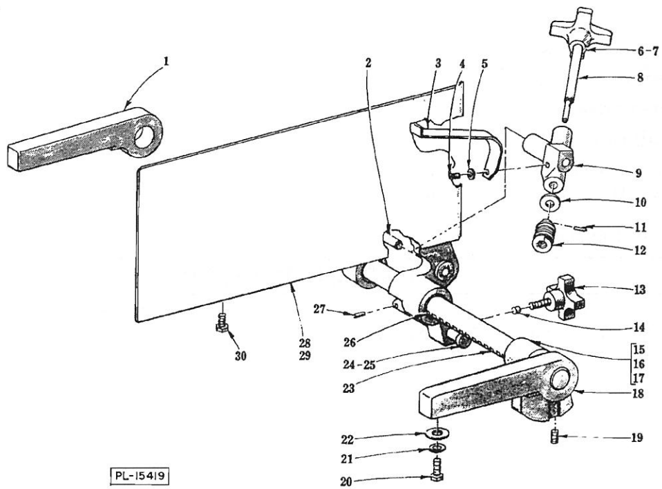
GAUGE PLATE UNIT
