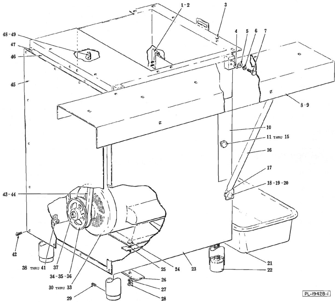
BASE UNIT
