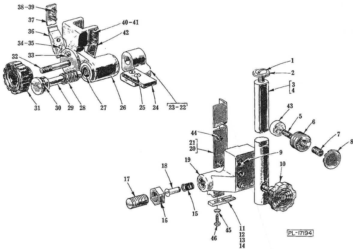
UPPER GUIDE AND PULLEY WIPER UNIT
